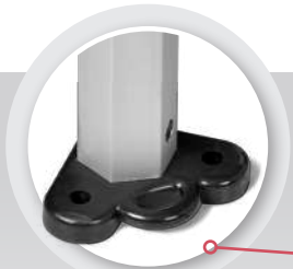
Aluminium hexagonal leg profile for superior strength & pre-punched feet to easily secure gazebo with ground pegs
